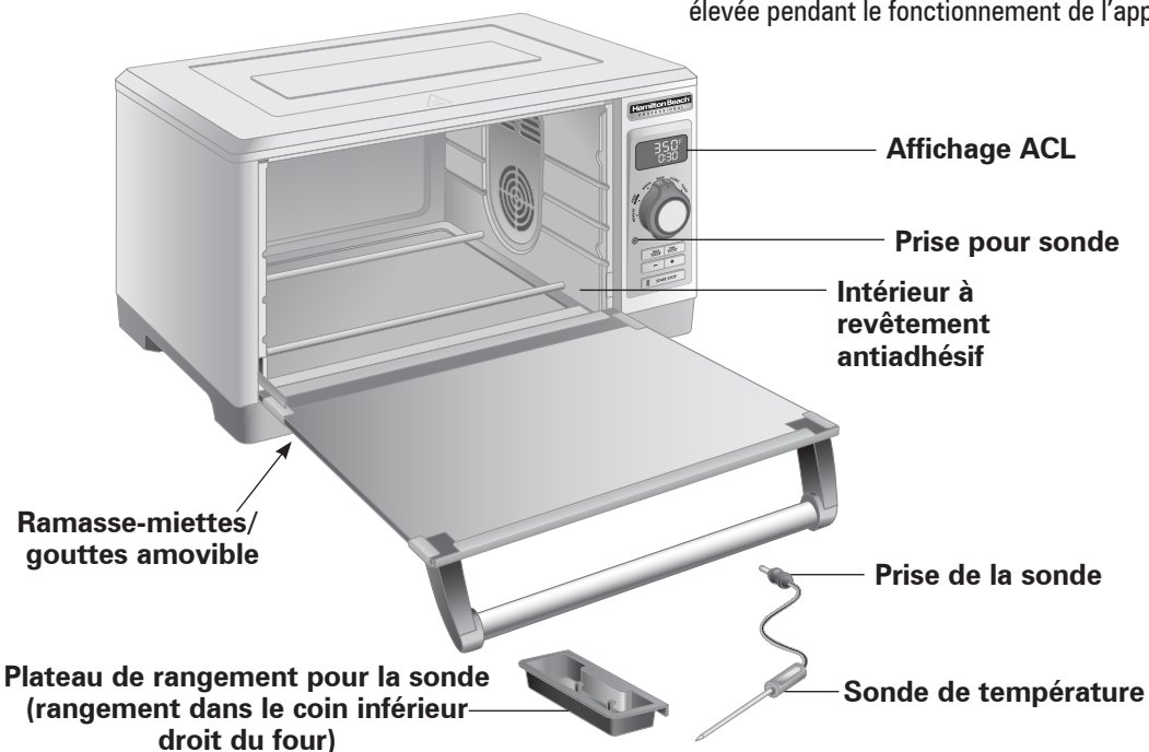
Ramasse-miettes/gouttes amovible
